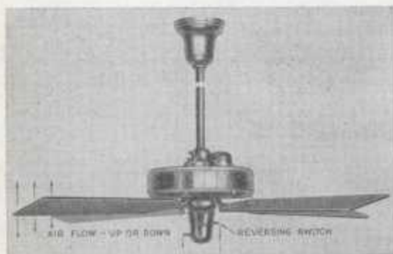
52-INCH—REVERSIBLE—AIR FLOW UP OR DOWN For Alternating Current 115 Volts, 60 Cycles. 3 Speeds
