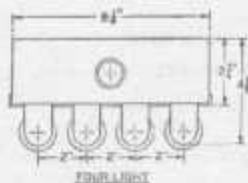
Dimensions of Four-Light Channels
